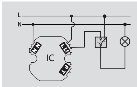
ⒾⒸ INFRAcontrol ⊗ Licht Ⓜ Motor
