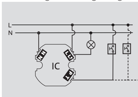
ⒾⒸ INFRAcontrol ⊗ Licht Ⓜ Motor
